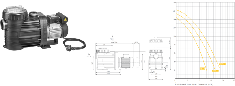
BADU Top II 8m3/h H=8m 0,30kW/230V
