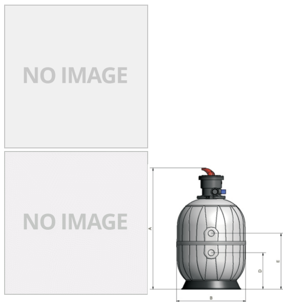
Aquarius TOP Ø450 6m 3 /h 1 1/2"
